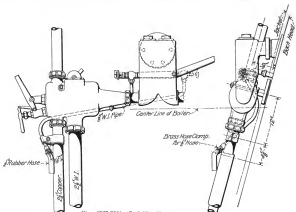
Figs. 2963-2964. Sprinkler Hose Connection.
